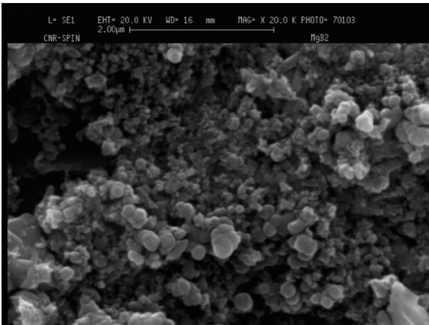
MgB 2 synthesized reacting magnesium and lab-made boron
